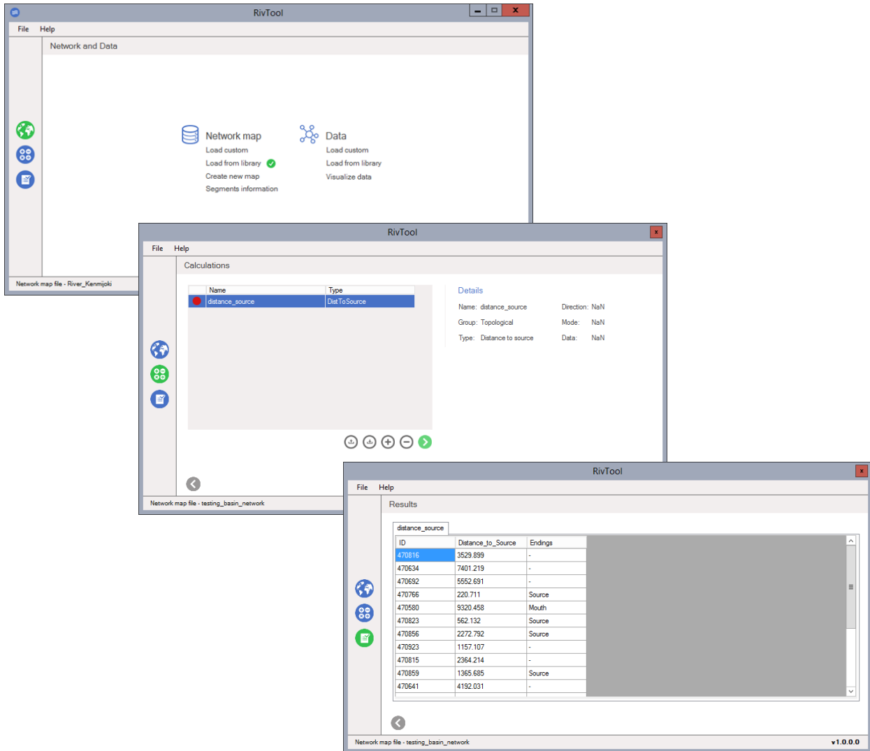
Figure 1 – Snapshots of the River Network Toolkit interface. From top to bottom: first, second and third window.
